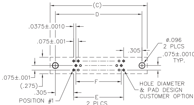
PCB LAYO VIEWED FROM COMPONENT SIDE
